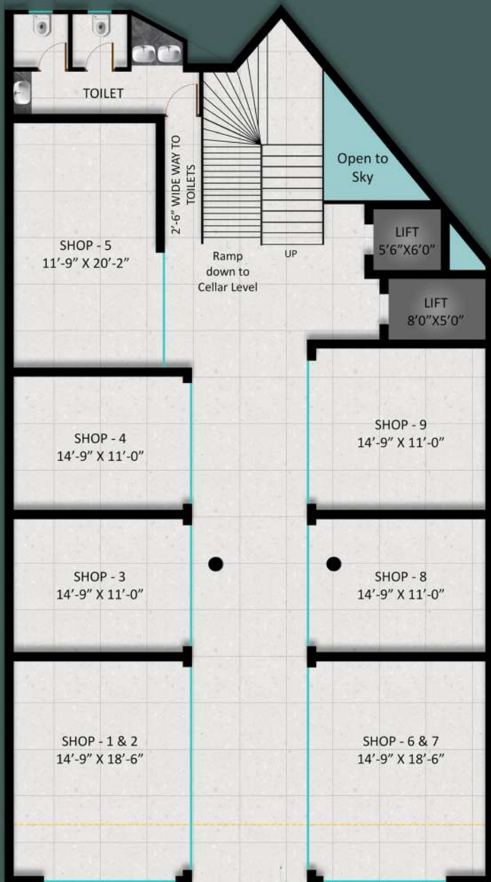
SECOND FLOOR & THIRD FLOOR PLAN
